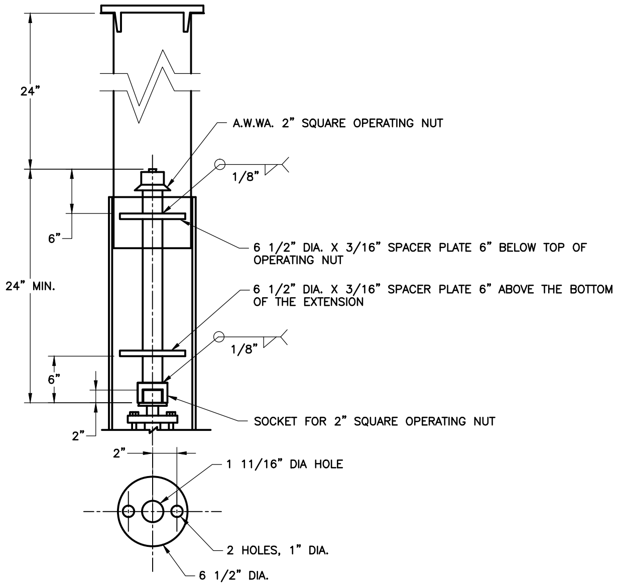
SPACER PLATE PLAN
