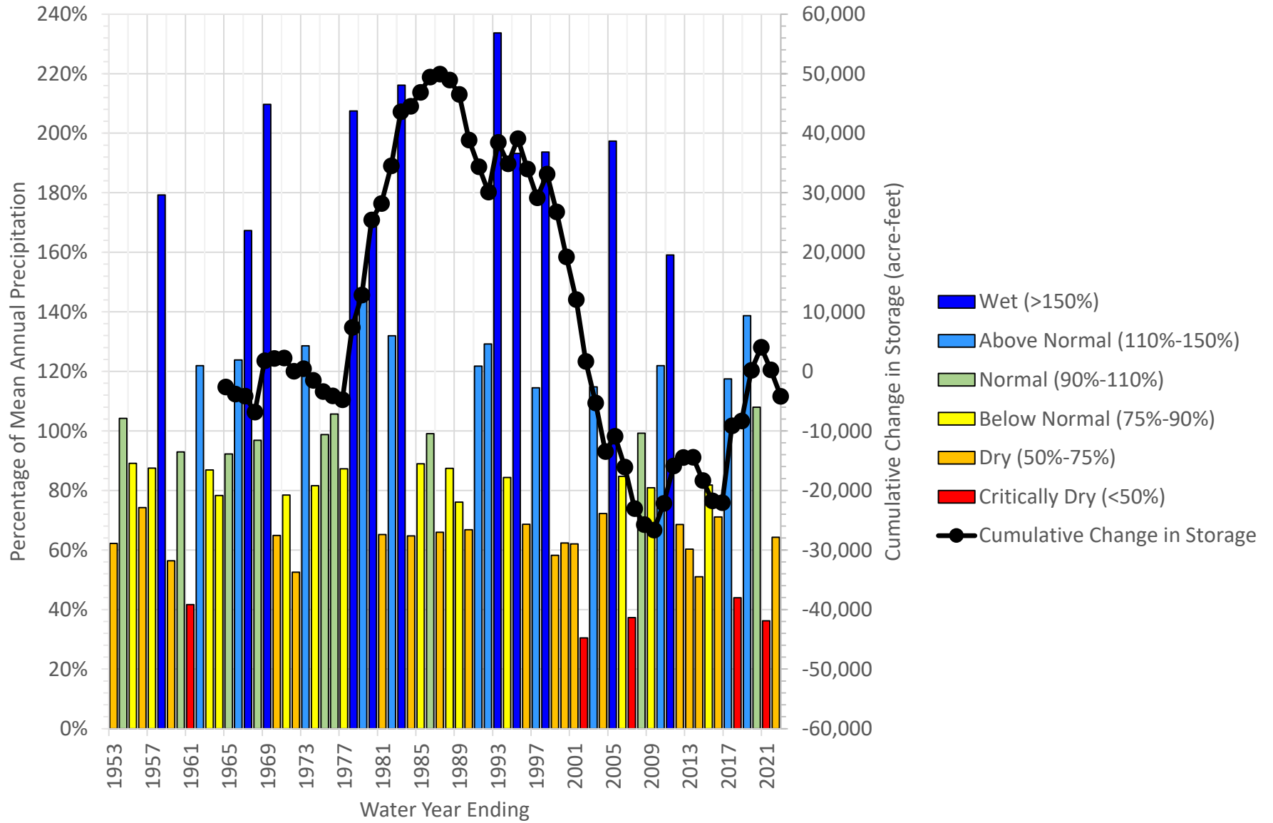
Figure 13. Historical Water Year-Types and Cumulative Change in Storage in the Yucaipa Subbasin
