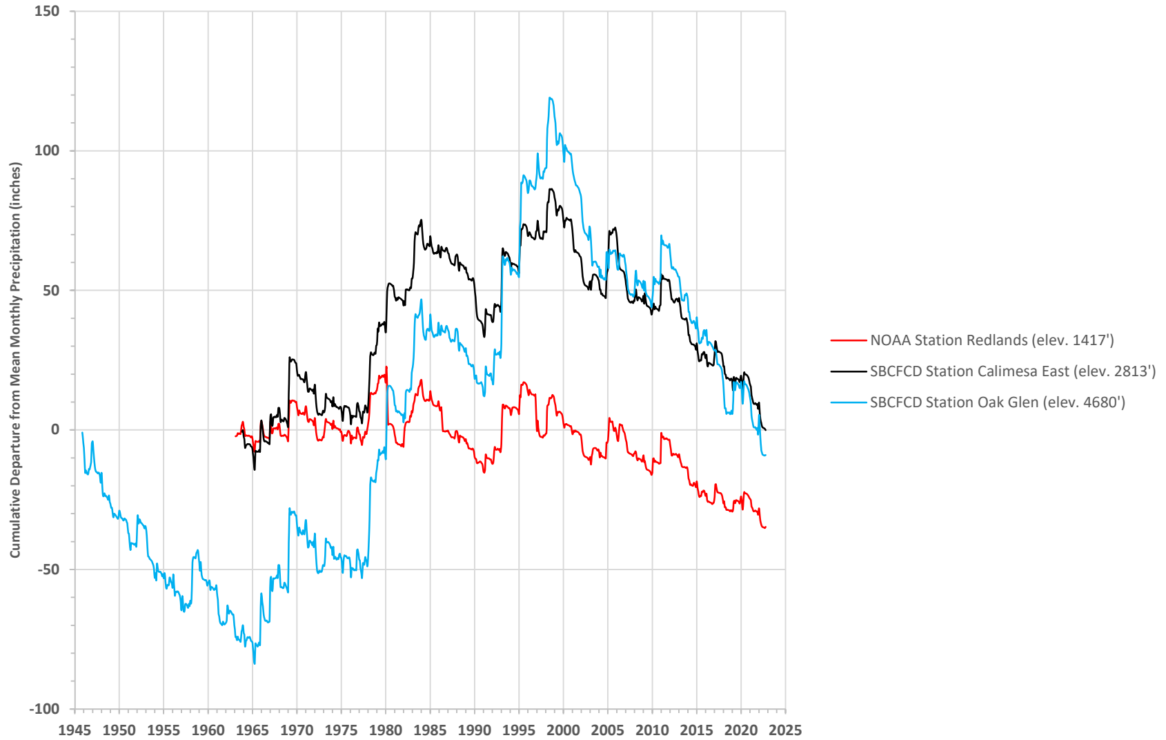
Figure 7. Cumulative Departure from Mean Monthly Precipitation at the SBCFCD Oak Glen and Calimesa East Climatic Stations and the NOAA Redlands Climatic Station
