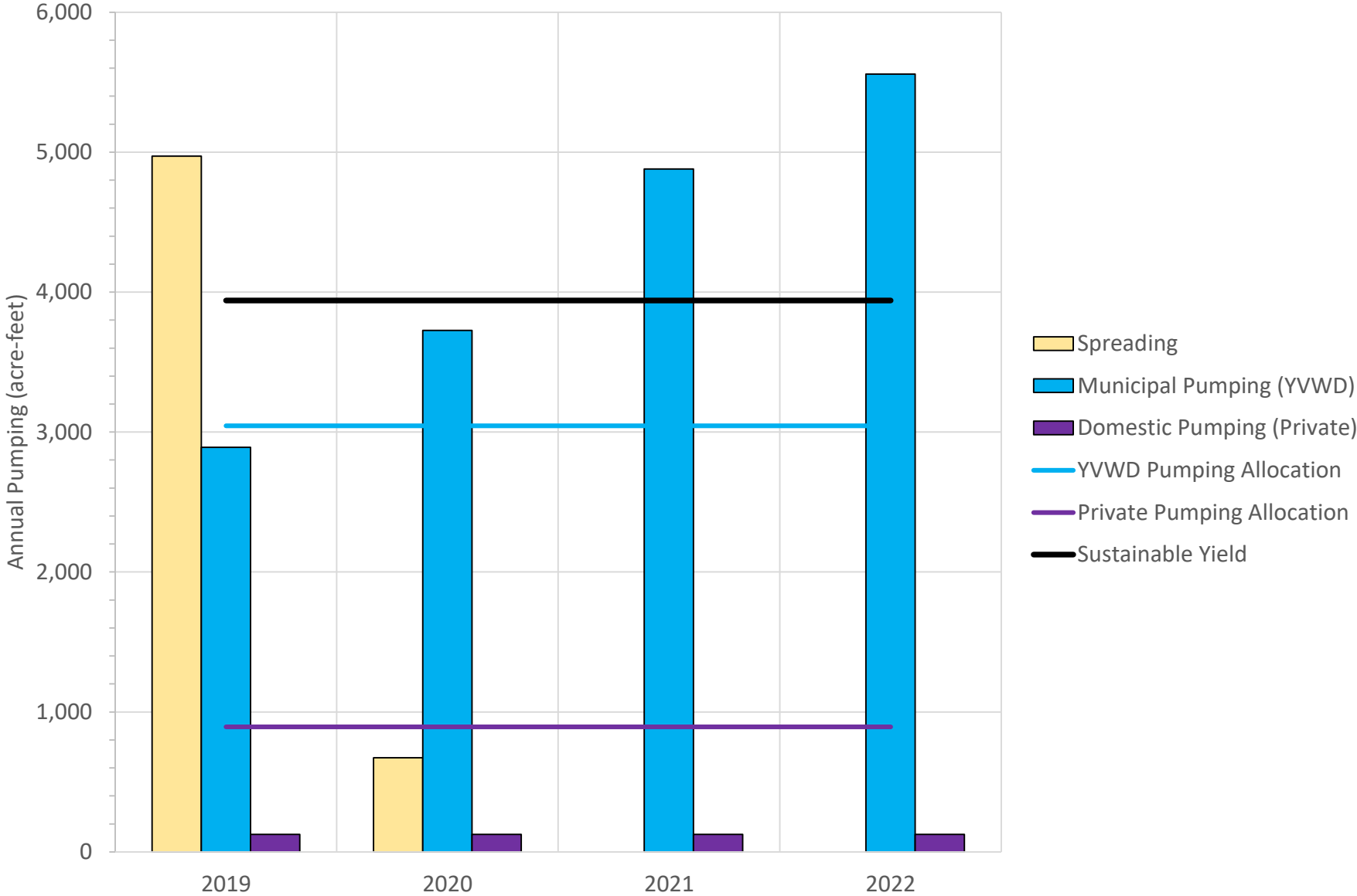
Figure 15. Annual Pumping and Spreading in the North Bench Management Area for the 2019-2022 Water Years
