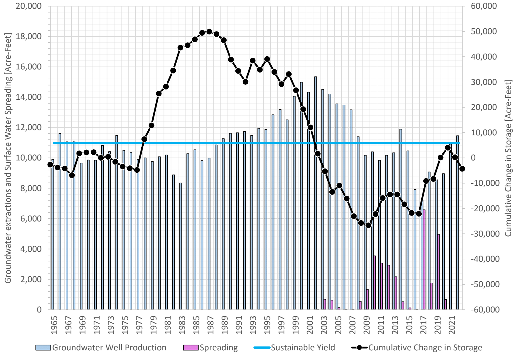
Figure 12. Annual Change in Groundwater in Storage in the Yucaipa Subbasin
