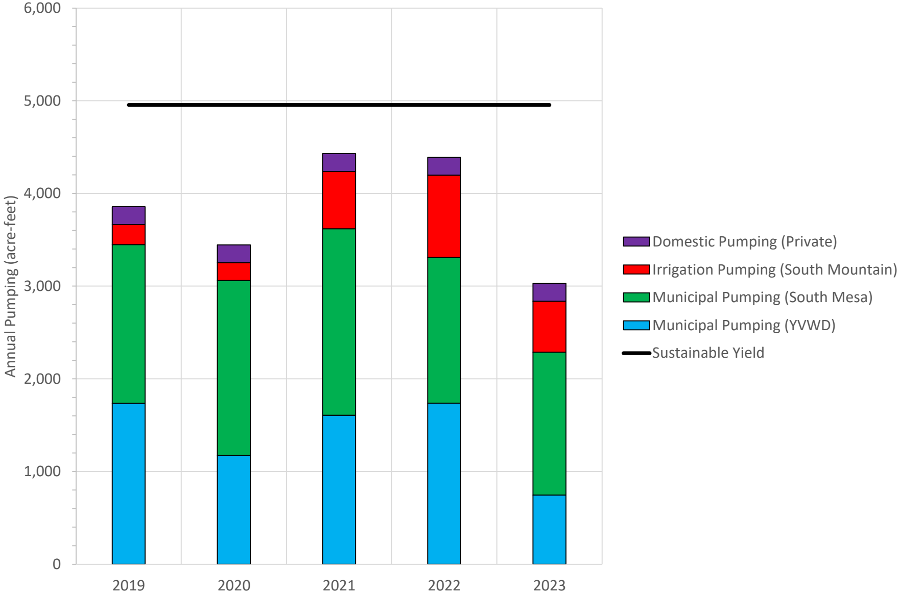
Figure 18. Annual Pumping in the Calimesa Management Area for the 2019 - 2023 Water Years
