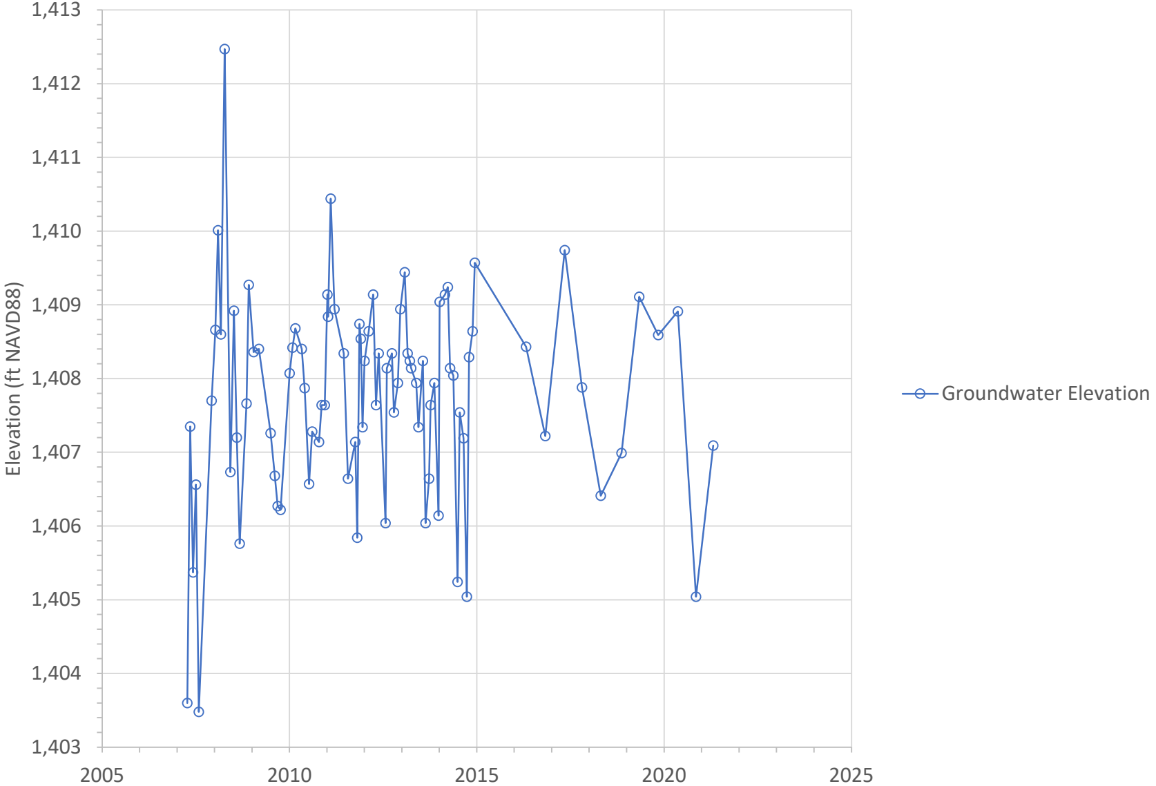
Groundwater Elevation at GL-8 in the San Timoteo Management Area
