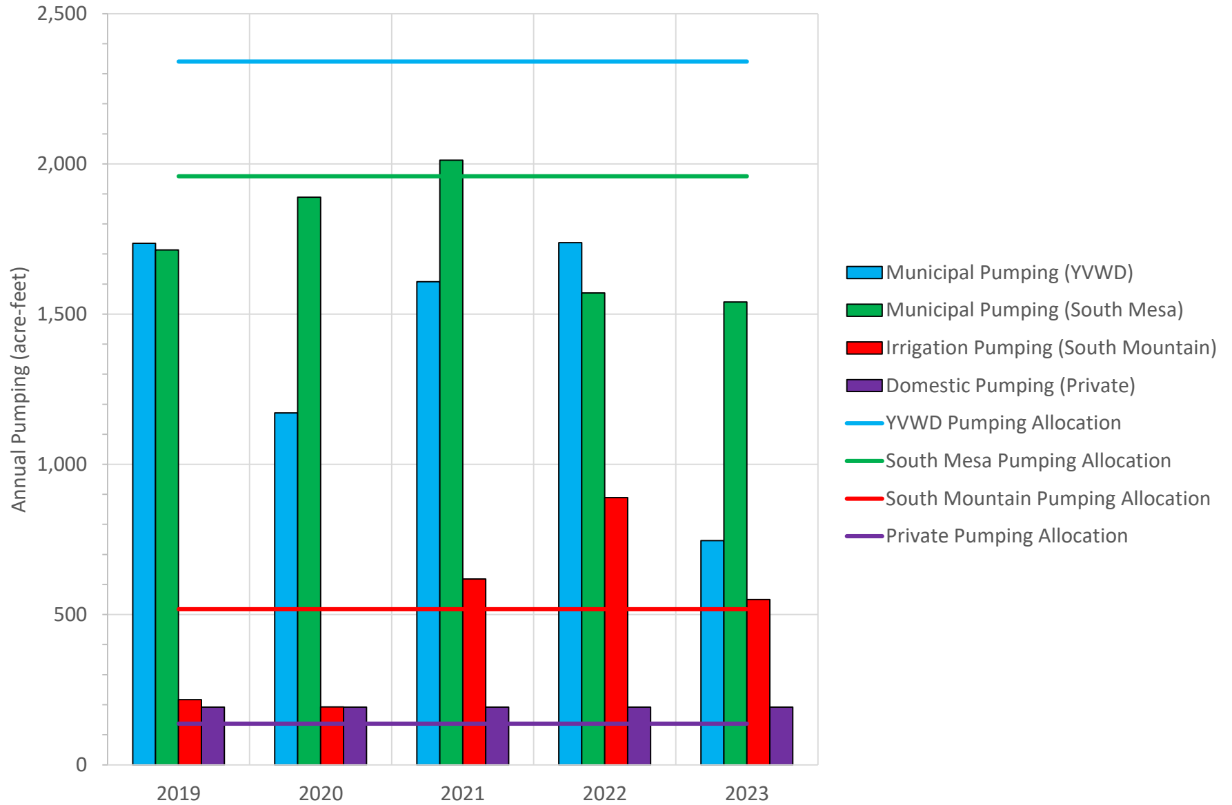
Figure 17. Annual Pumping by User in the Calimesa Management Area for the 2019 - 2023 Water Years
