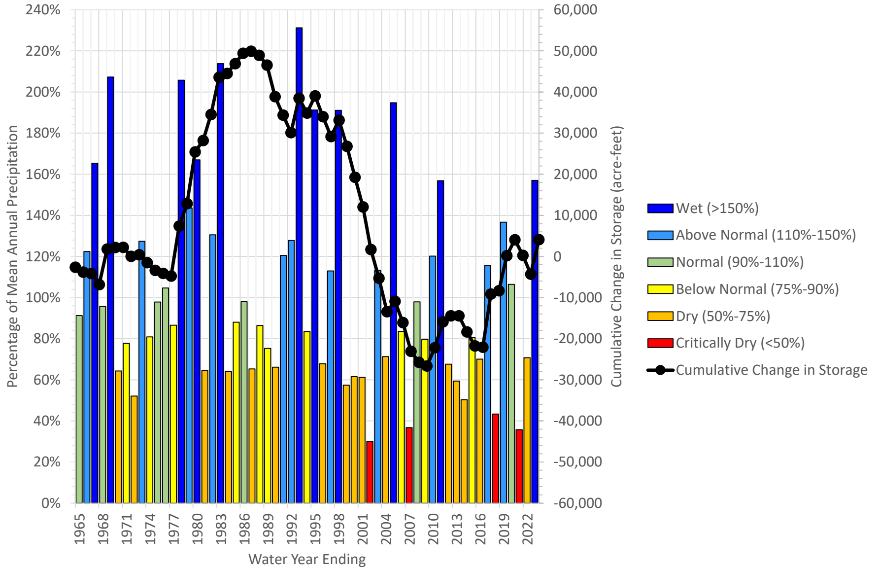
Figure 14. Historical Water Year-Types and Cumulative Change in Storage in the Yucaipa Subbasin
