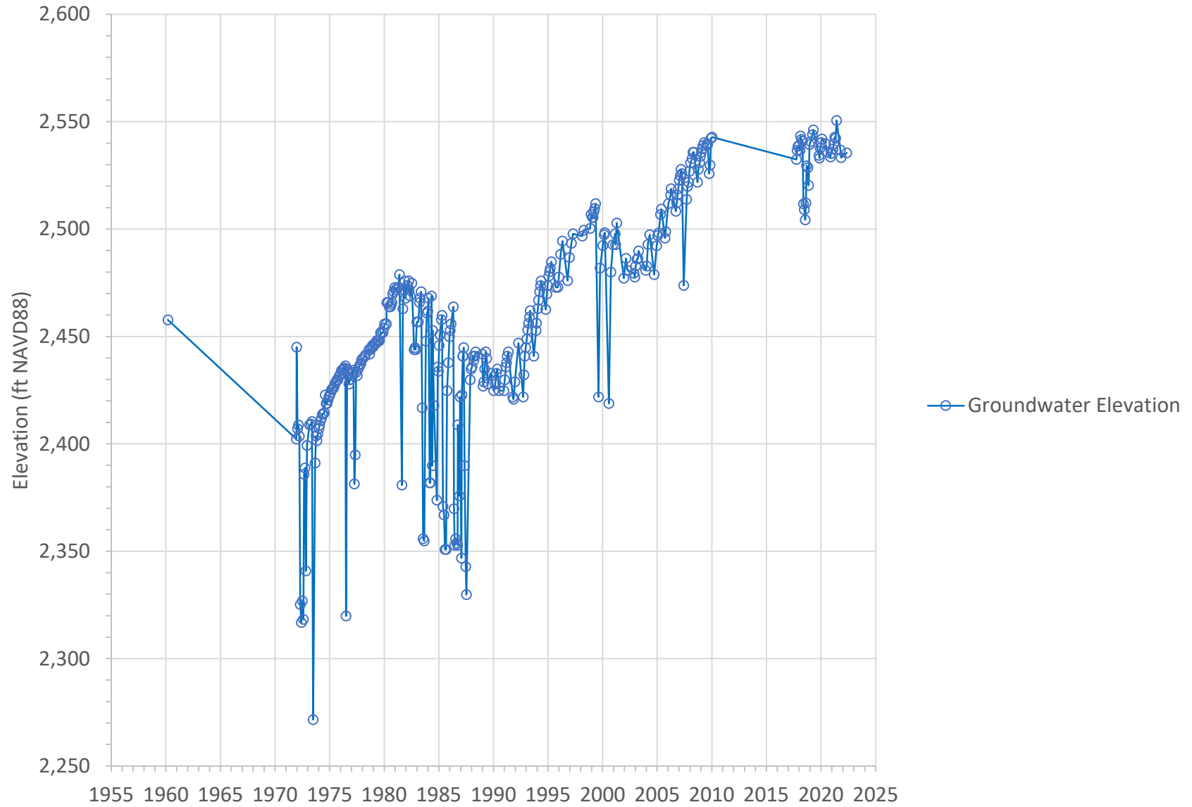
Groundwater Elevation at YVWD-09 in the North Bench Management Area
