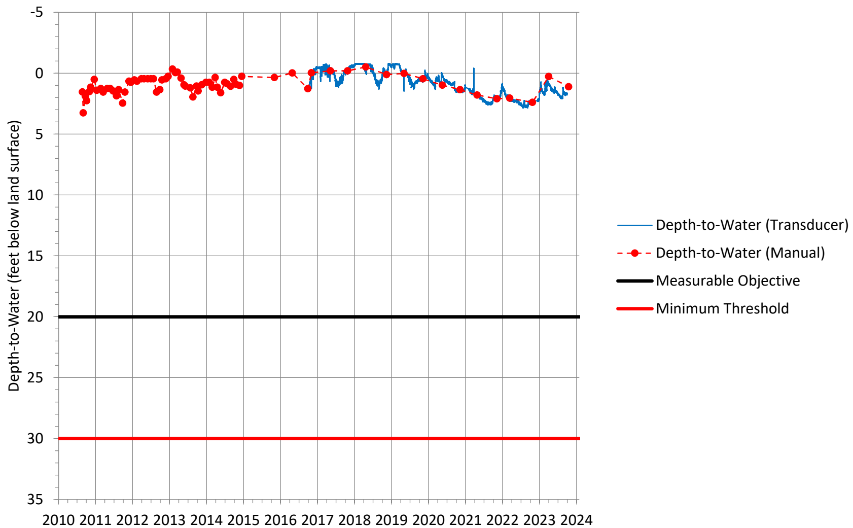
Depth-to-Water Well YVWD GMMW-5B in the San Timoteo Management Area
