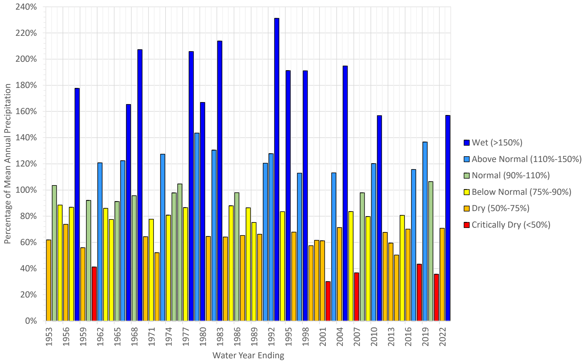
Figure 9. Historical Water Year-Types in the Yucaipa Subbasin
