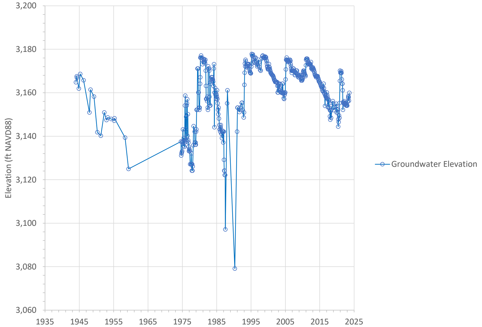
Groundwater Elevation at YVWD-13 in the North Bench Management Area
