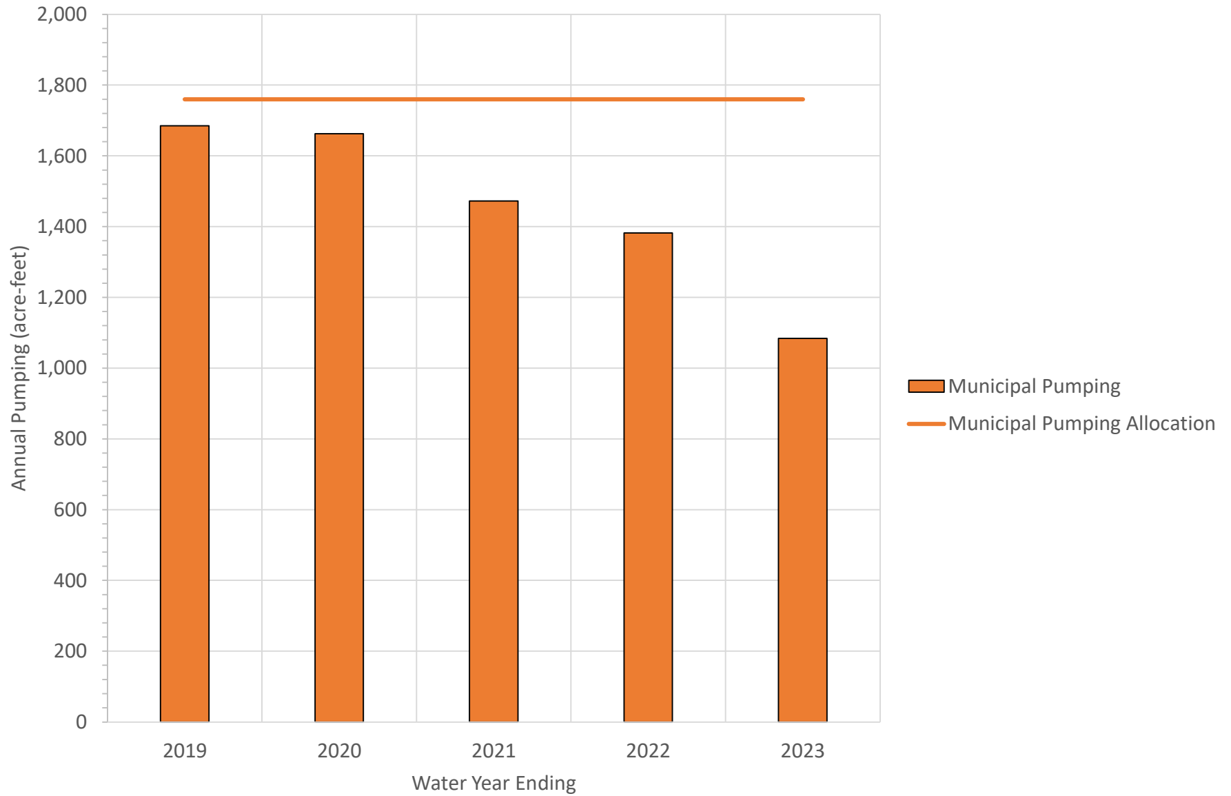
Figure 19. Annual Pumping in Western Heights Management Area for 2019 - 2023 Water Years
