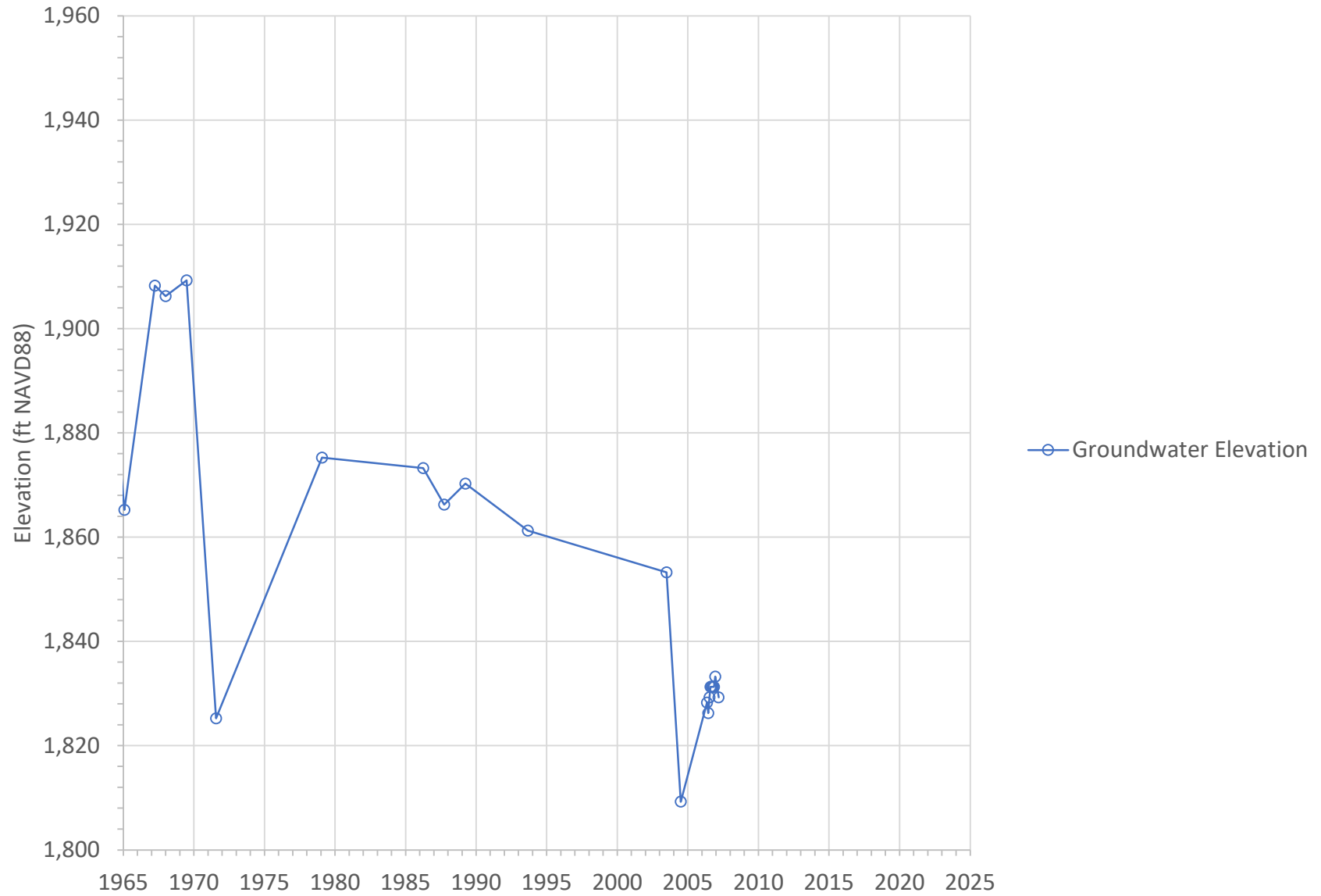
Groundwater Elevation at WHWC-09 in the Western Heights Management Area
