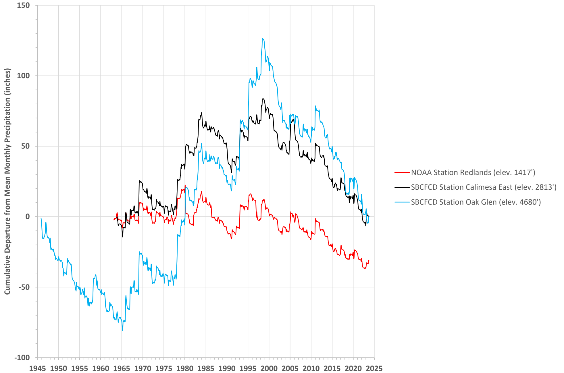
Figure 8. Cumulative Departure from Mean Monthly Precipitation at the SBCFCD Oak Glen and Calimesa East Climatic Stations and the NOAA Redlands Climatic Station
