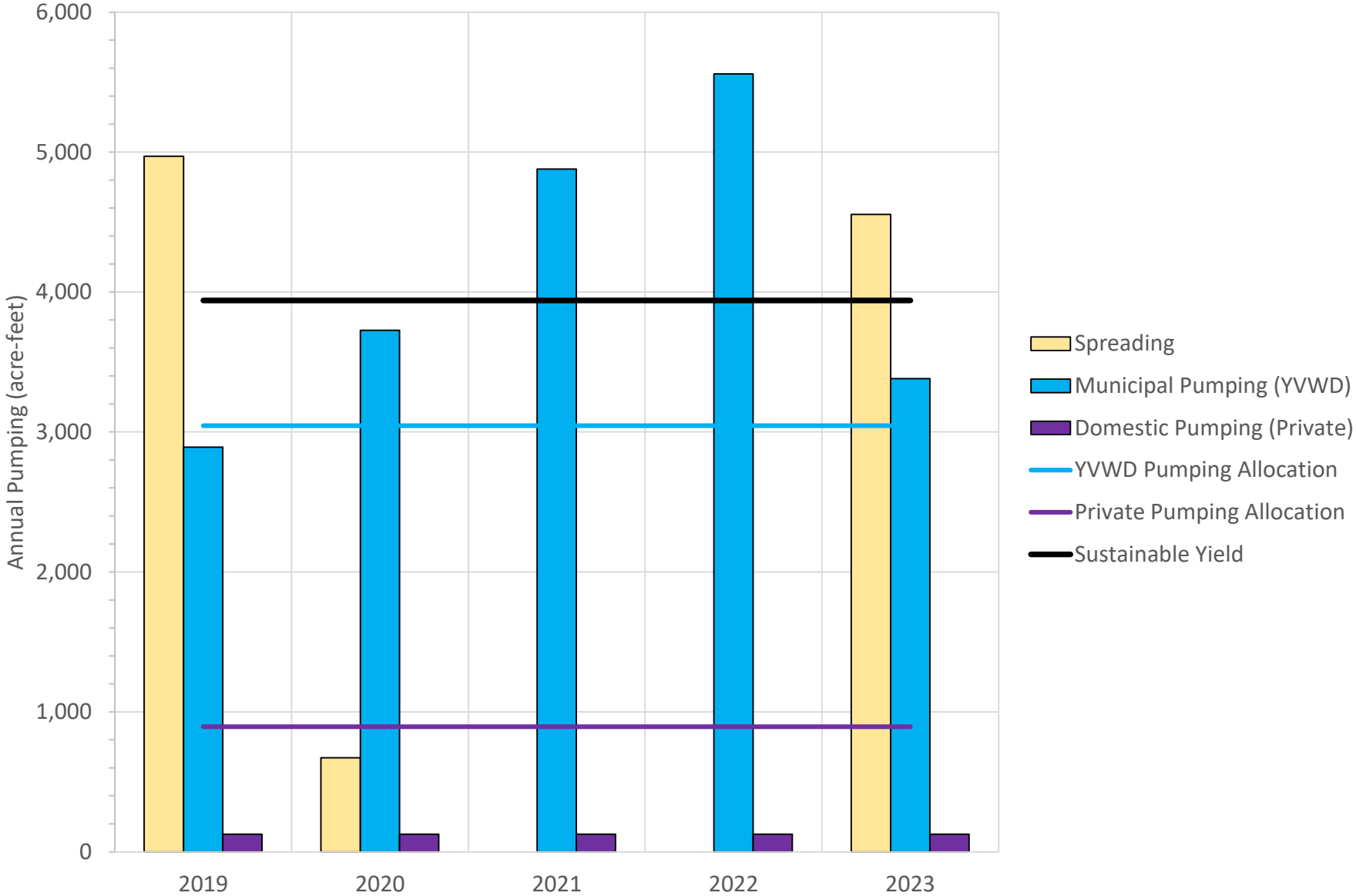
Figure 16. Annual Pumping and Spreading in the North Bench Management Area for the 2019-2023 Water Years
